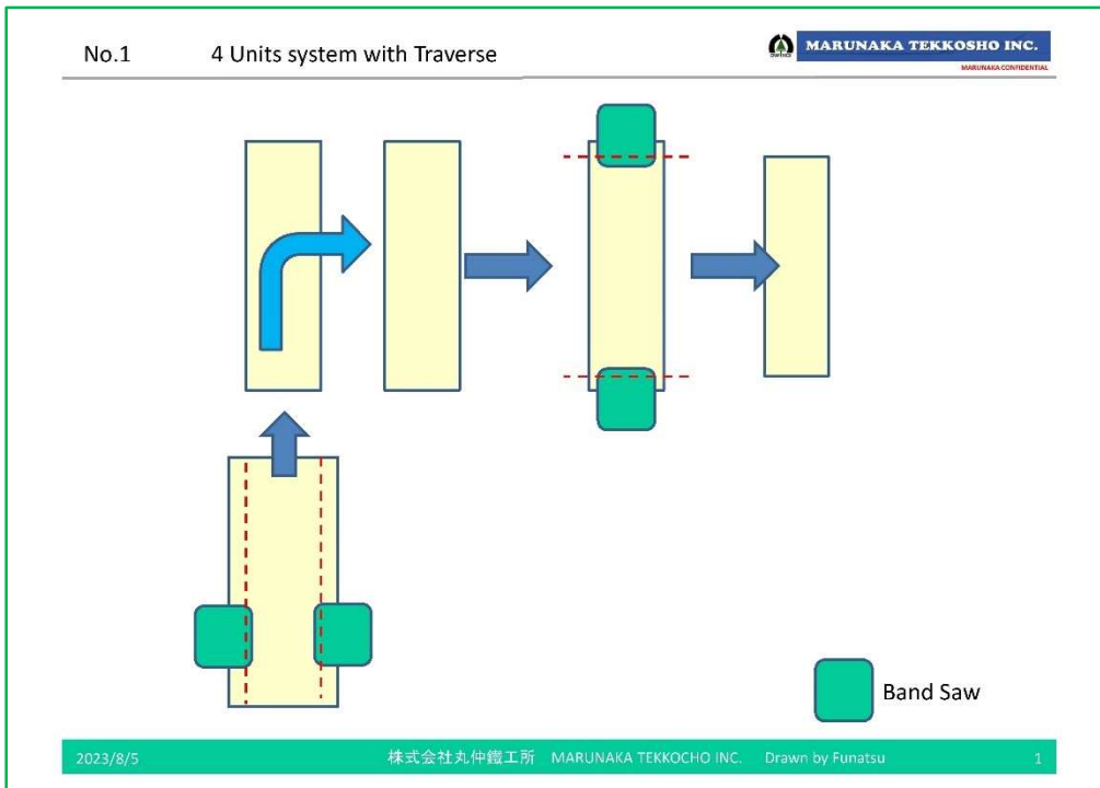
No. 1 – Concept consisting of two (2) Twin Bandsaw sets incl. Auto-Angular-Transfer Section
