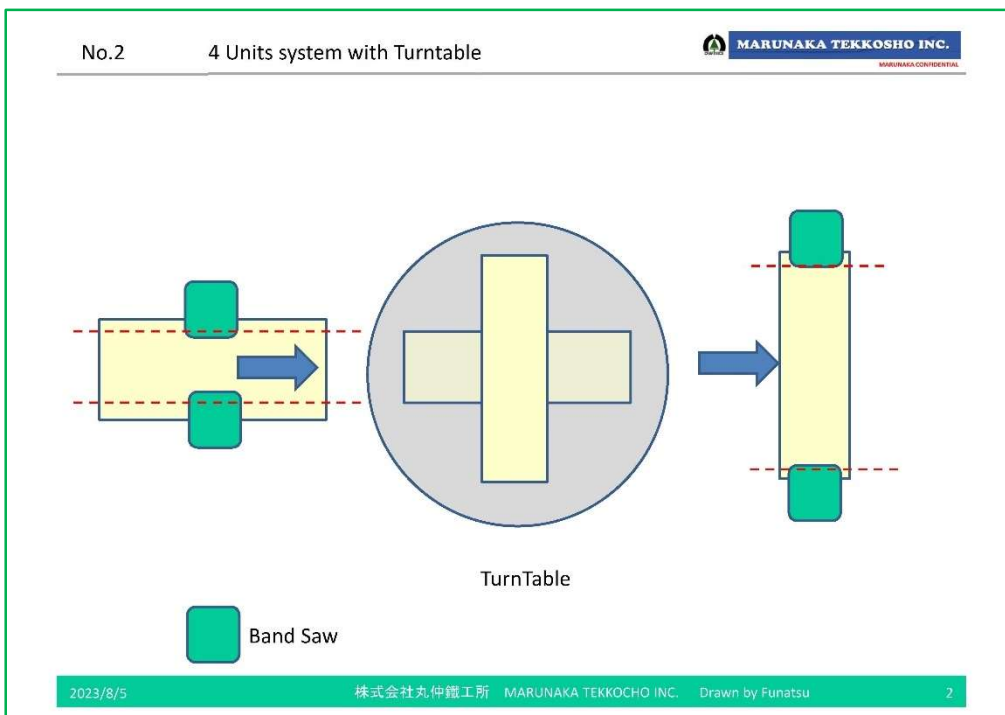
No. 2 – Concept consisting of two (2) Twin Bandsaw sets incl. Auto-Turn-Table Section
